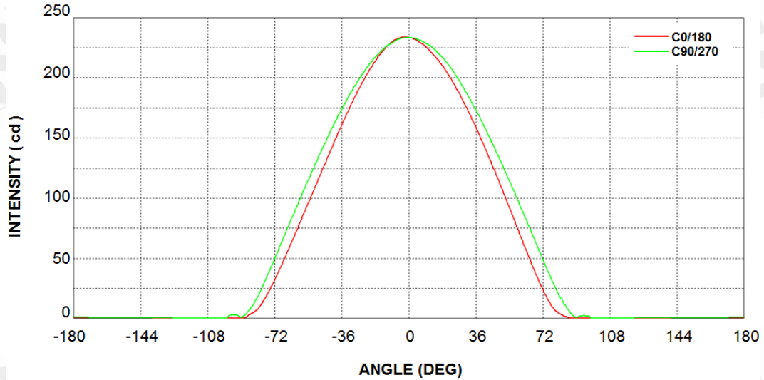
LUMINOUS INTENSITY DISTRIBUTION DIAGRAM
